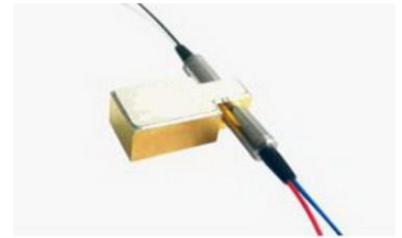
2×2 MM Optical Switch
